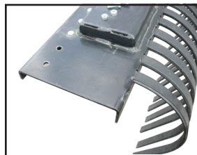
Figure 1 - Remove two (2) outer bolts holding tines.
